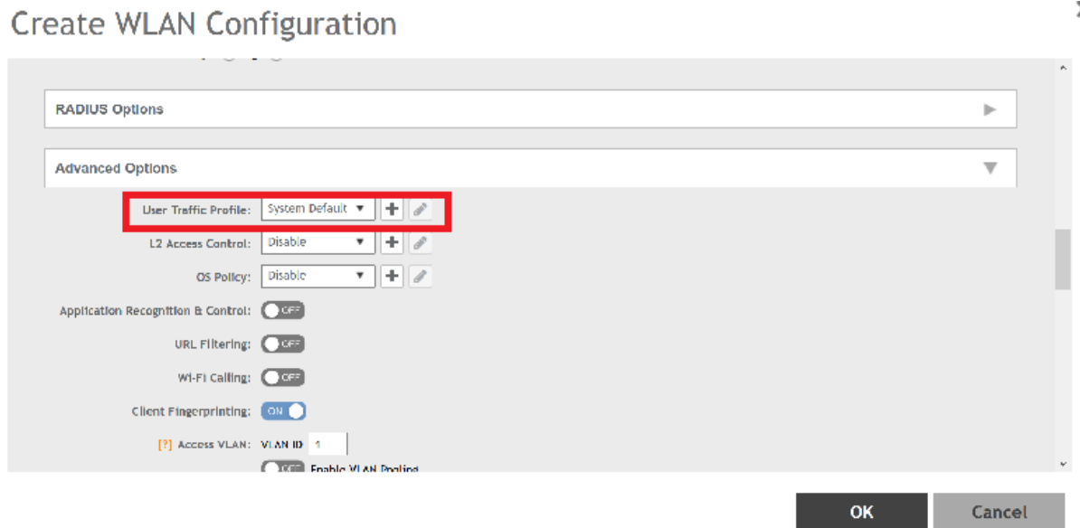
FIGURE 163 Apply the UTP to a WLAN
