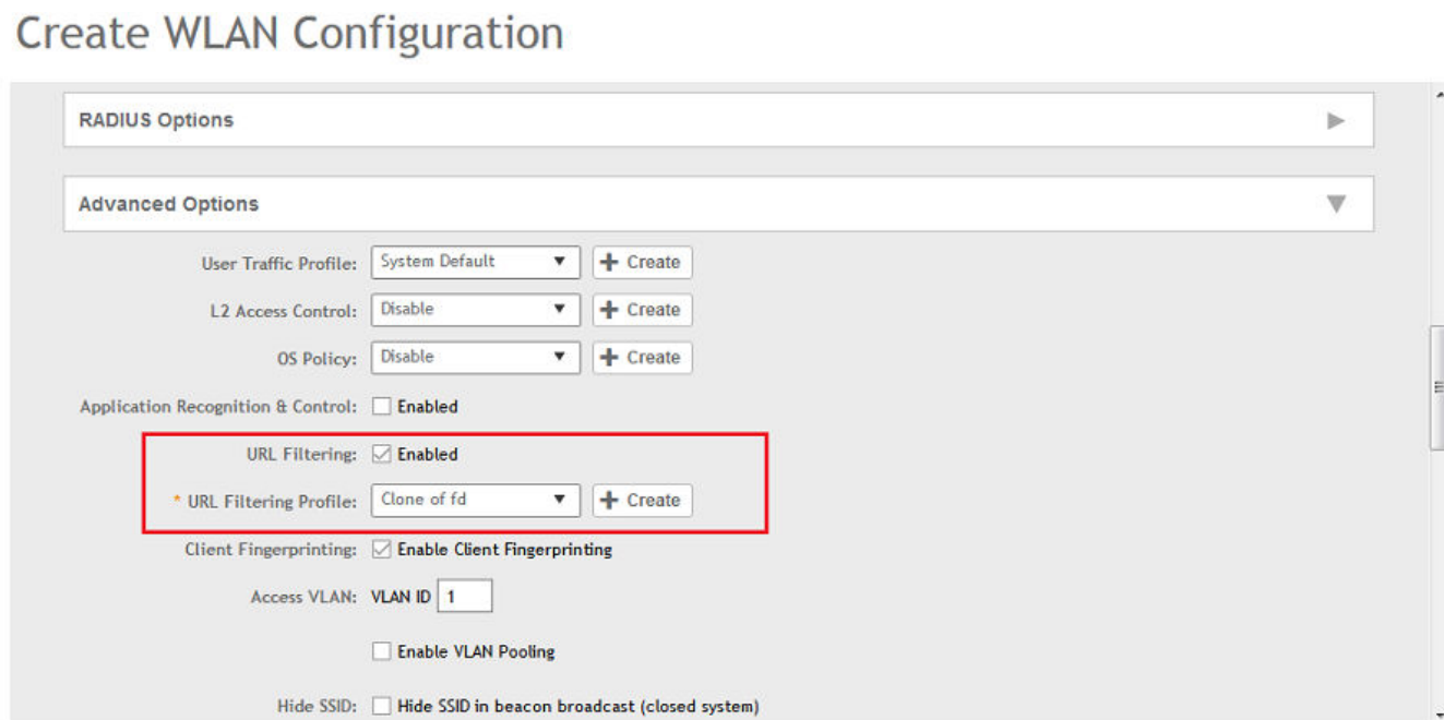
FIGURE 167 Enabling URL Filtering
