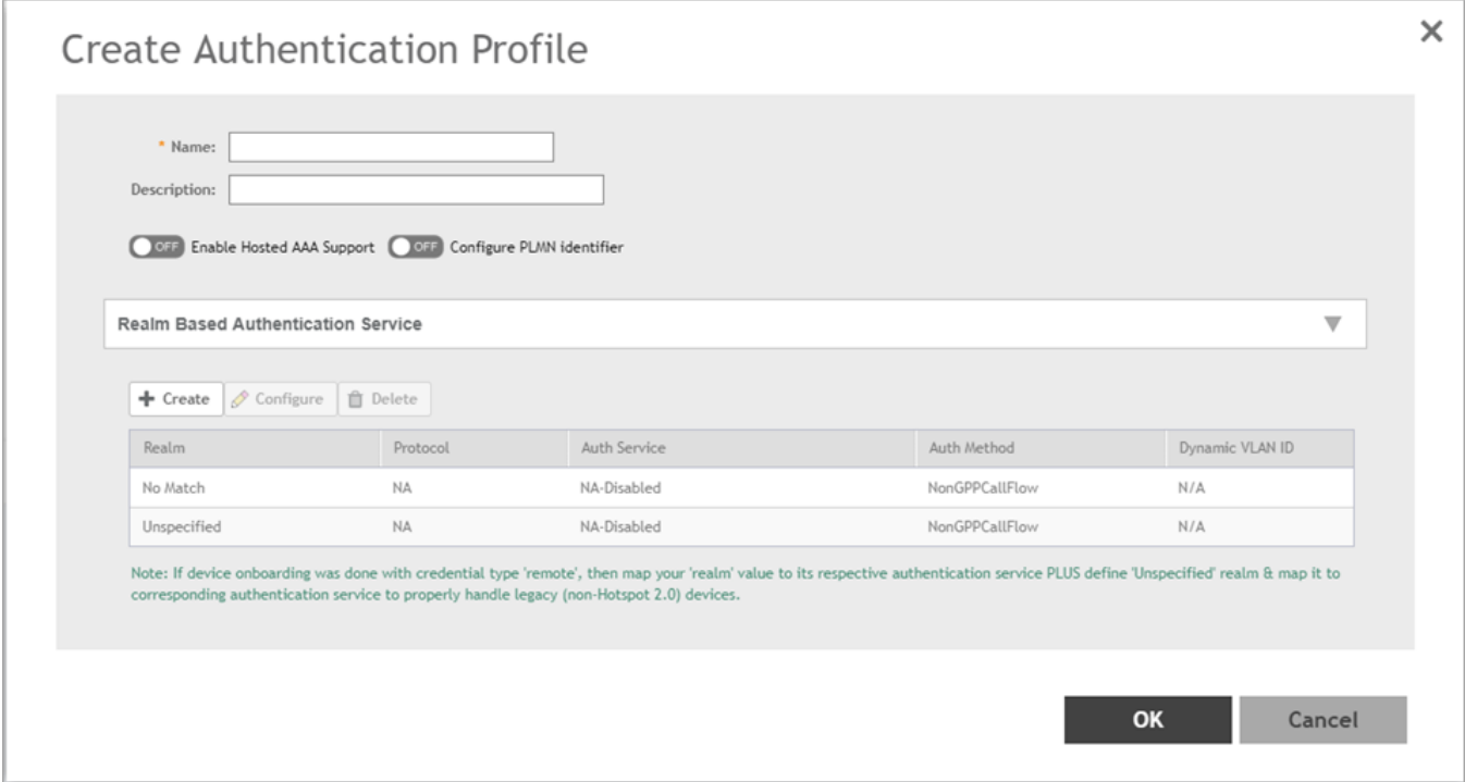
FIGURE 178 Creating a Realm Based Proxy Authentication Profile
